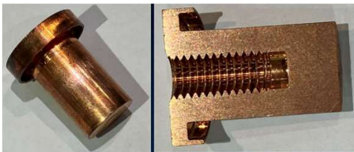
Relay Terminal
