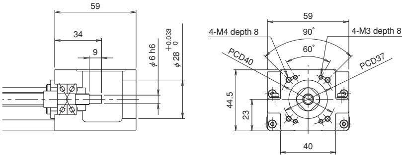
Motor bracket configuration: R0
