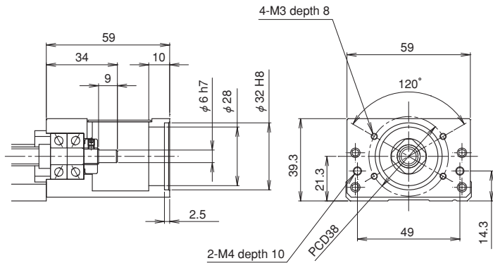
Motor bracket configuration: A0
