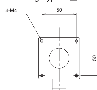
Dimensions of parallel motor mounting Type G□
