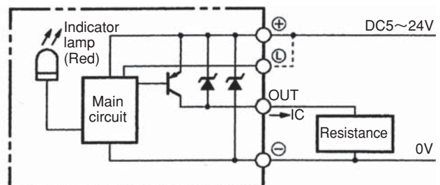
PNP output type
