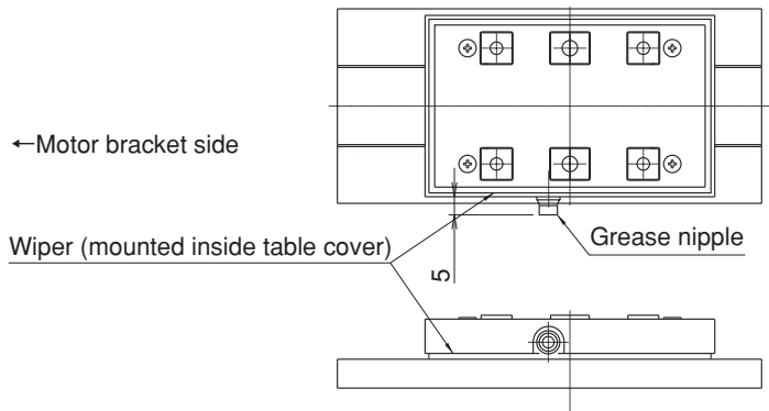
Full-cover type with grease nipple and wiper (Symbol: D)
