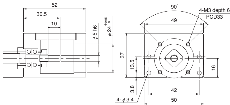
Motor bracket configuration: A0
